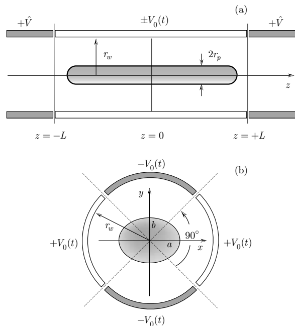
Figure 1: (a) Side view and (b) end view of Paul Trap Simulator Experiment (PTSX).
