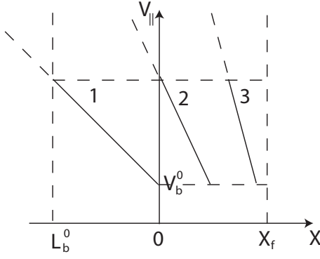
FIG. 1: Longitudinal phase space (x, v_{\parallel}) for the beam ions at different times during the longitudinal compression.
