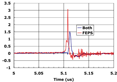
Figure 3: Time trace of the longitudinally compressed ion beam with charge neutralization with the FEPS and with both plasma sources
