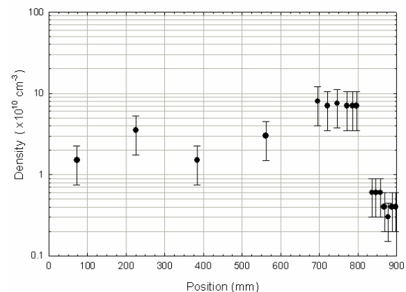
Figure 2: Density measurements along the axis of the \text{BaTiO}_3 FEPS indicate that the five sources are balanced in the mid- 10^{10} \text{cm}^{-3} density range.
