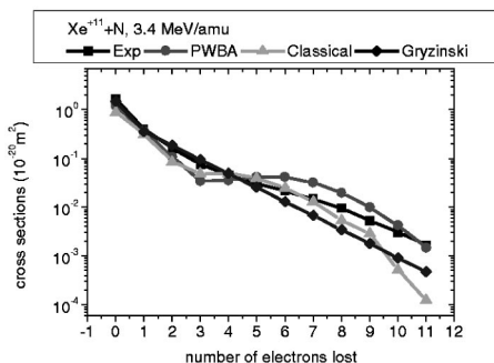
FIG. 3. Average cross sections for electron loss from 3.4 MeV/amu Xe^{11+} in N_2 per one nitrogen atom determined from the data taken at cell pressures \leq 8 mTorr.
