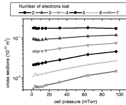
FIG. 4. Cross sections determined for the loss of two through seven electrons as a function of pressure for Kr^{7+} . Note that below about 10 mTorr, the data are insensitive to pressure, the thin-cell approximation is justified, and single collisions are the dominant process.
