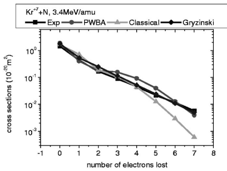
FIG. 2. Average cross sections for electron loss from 3.4 MeV/amu Kr^{7+} in N_2 per one nitrogen atom determined from the data taken at cell pressures \leq 8 mTorr.
